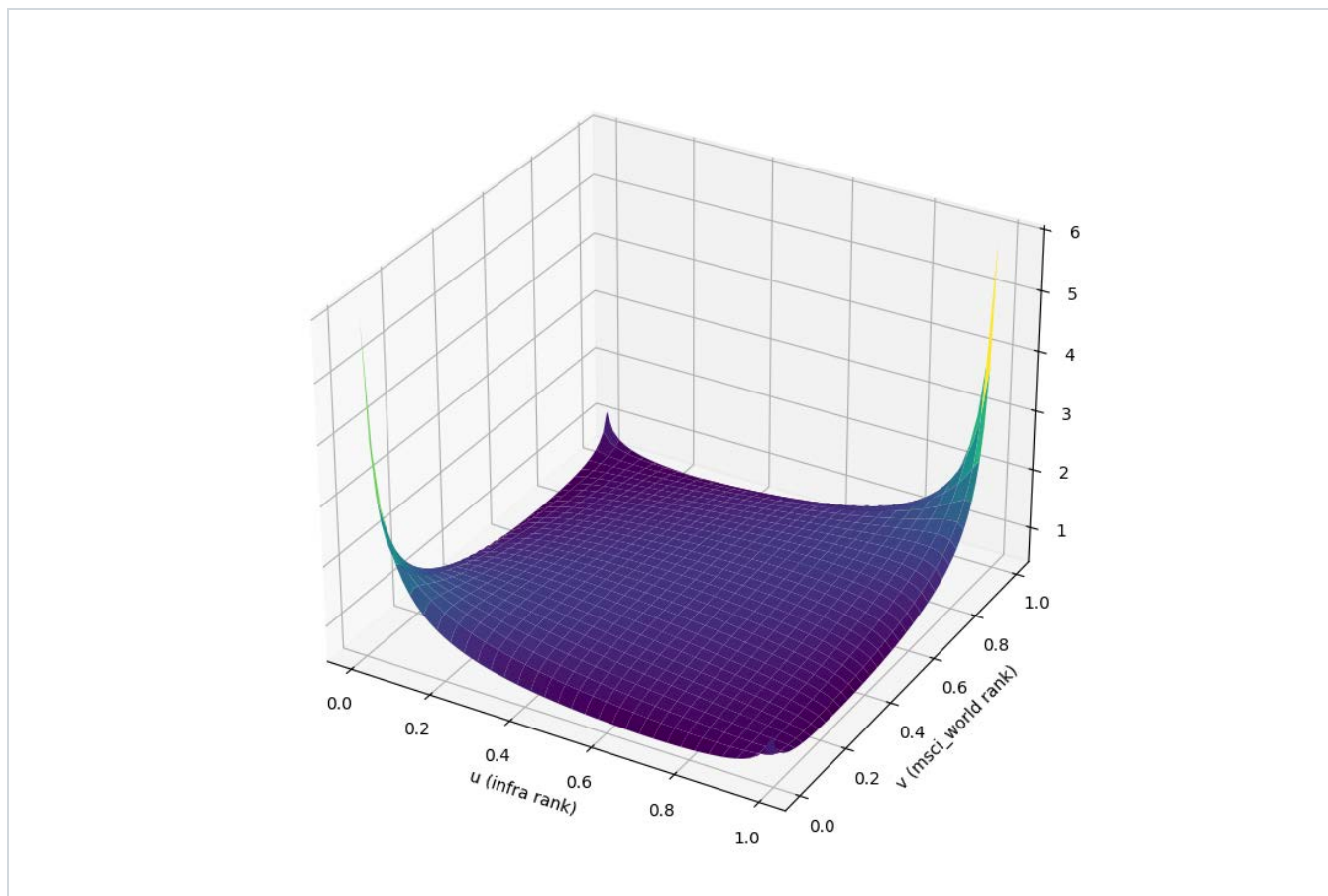
■ FIGURE 2 – INFRA300 EQUITY INDEX T-COPULA SURFACE
