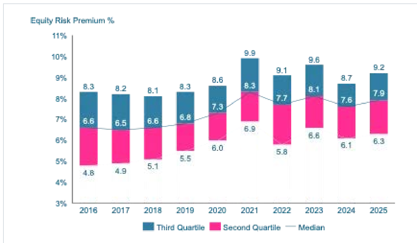
■ FIGURE 4 – INFRA300 VW INDEX EQUITY RISK PREMIA IQR
