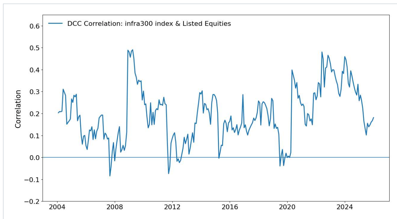
■ FIGURE 1 — INFRA300 EQUITY DYNAMIC CONDITIONAL CORRELATION WITH FAMA FRENCH (FF) MARKET FACTOR
